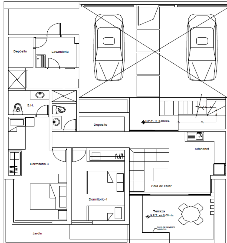
Main Floor
